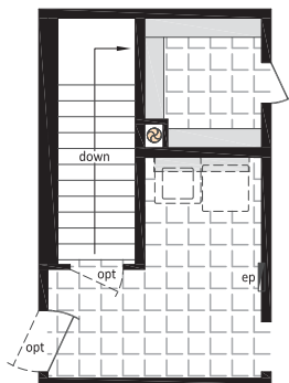
Proposed Stair Location for Optional Foundation Model
