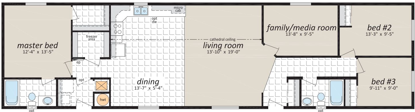
CJN-3011 , 20' x 76' - 1,520 sq. ft.
