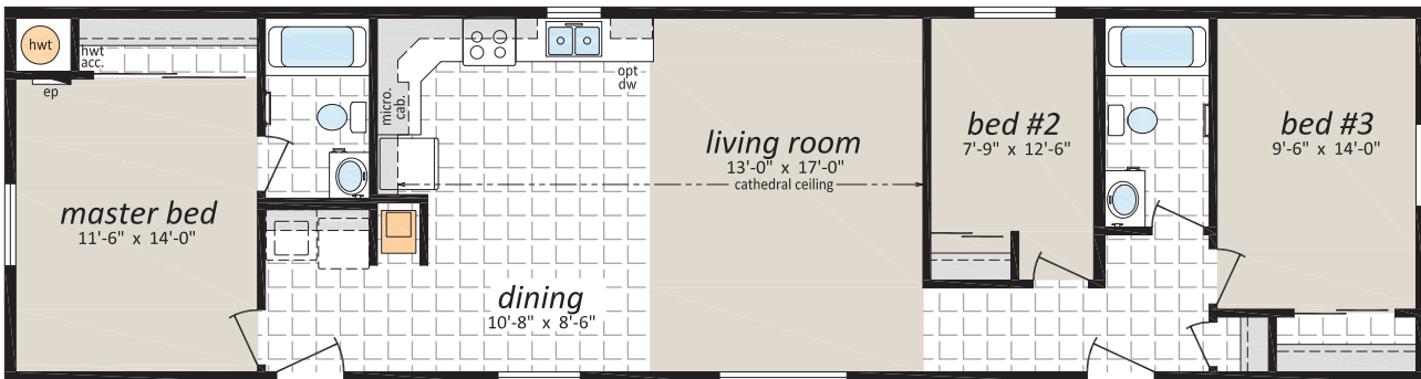
CJN-1845, 18' x 68' - 1,224 sq. ft.
